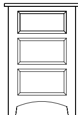
BN-21-[SH] Nightstand 3 Drawers 20w 19d 30h
