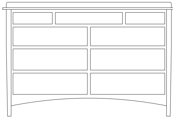
BD-944-[SR] Dresser 9 Drawers 71w 19d 48h
